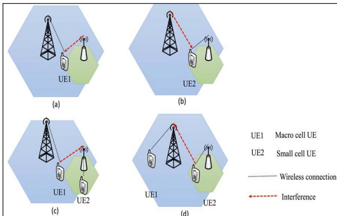
Figure 11: Multi-tier interference cases. Source: Authors, (2024).
