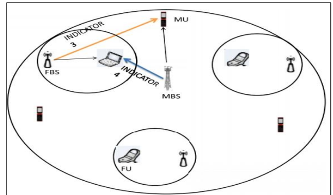
Figure 10: A typical cross-tier interference scenario between FBSs. Source: Authors, (2024).
