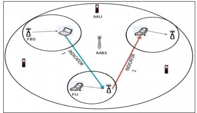
Figure 9: A typical co-tier interference scenario between neighboring FBSs. Source: Authors, (2024).
