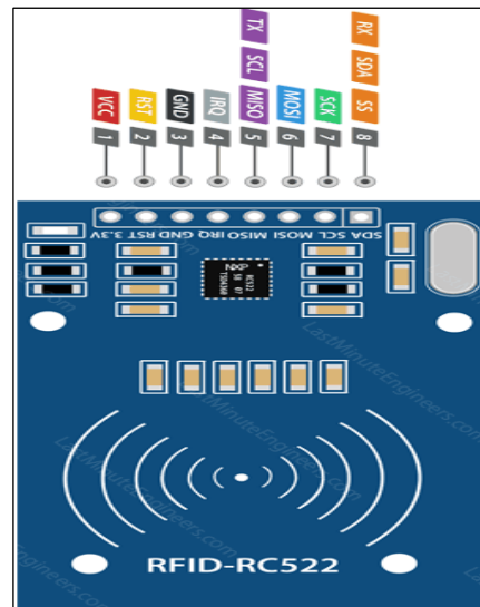
Figure 3: RC522 RFID Reader. Source: [21].
