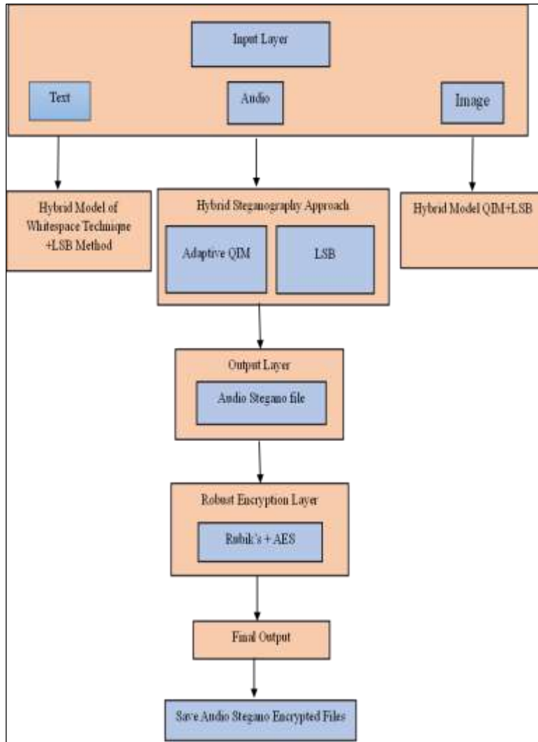
Figure 1: Hybrid Audio Security Process Flow Diagram. Source: Authors, (2025).
