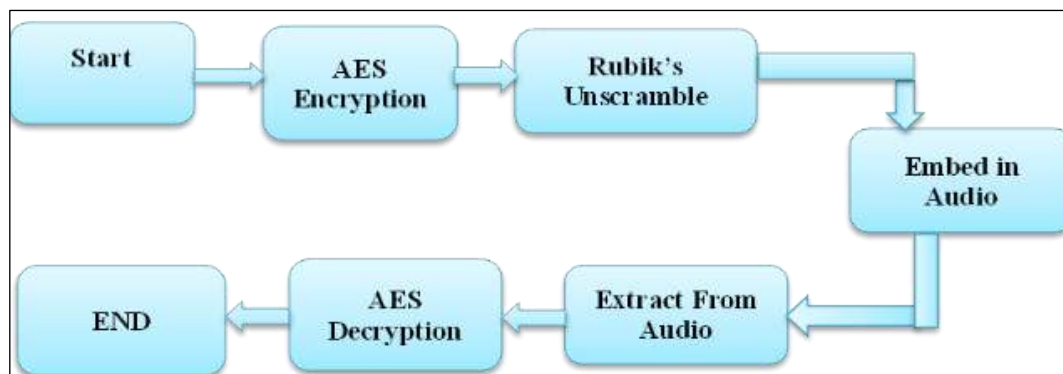
Figure 2: Robust Encryption Approach.
