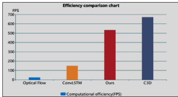
Figure 4: Efficiency Performance Comparison. Source: Authors, (2024).
